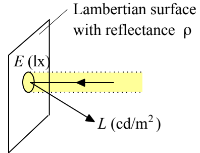
Figure 8. Relationship between illuminance and luminance
