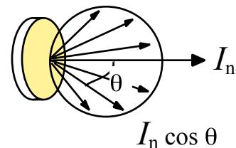
Figure 7. Lambert's cosine law
