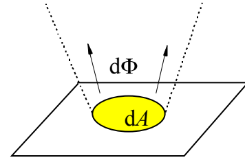
Figure 6. Radiant exitance and luminous exitance
